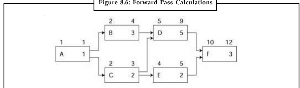
Figure 8.6: Forward Pass Calculations
