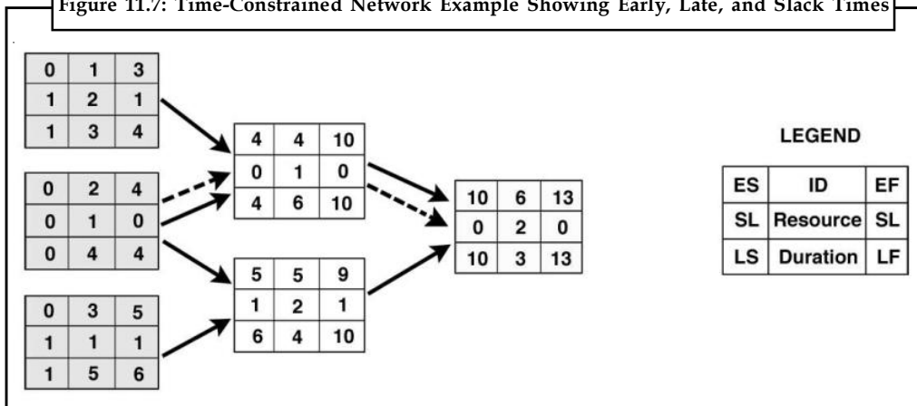
Figure 11.7: Time-Constrained Network Example Showing Early, Late, and Slack Times
