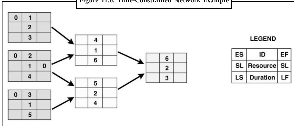
Figure 11.6: Time-Constrained Network Example
