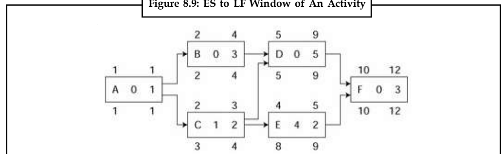
Figure 8.9: ES to LF Window of An Activity
